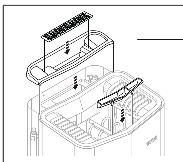
Figure 14: Fitting the cover for the water reservoir, herb grille and fragrance holder/air humidifier
