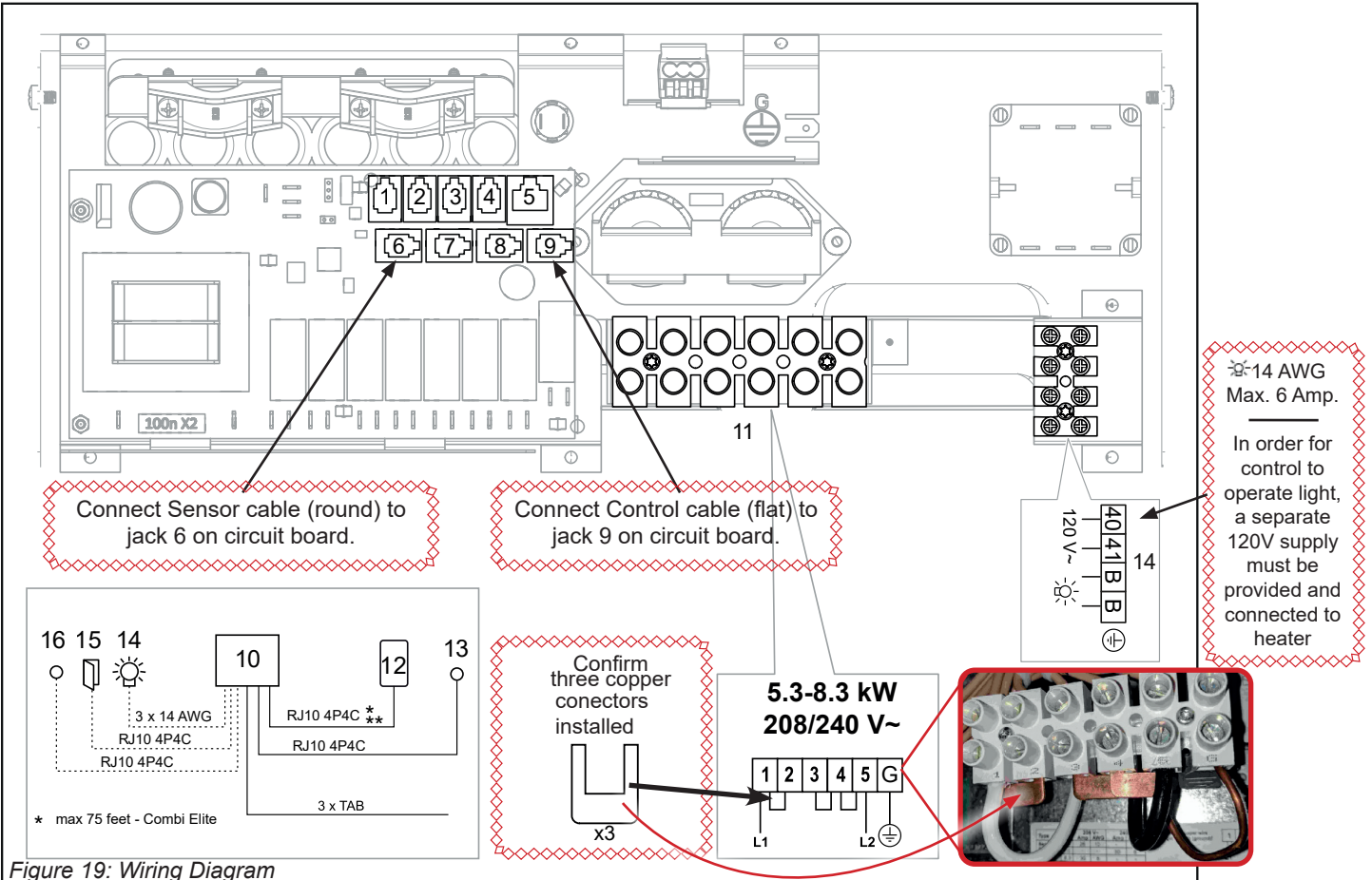
Figure 19: Wiring Diagram
