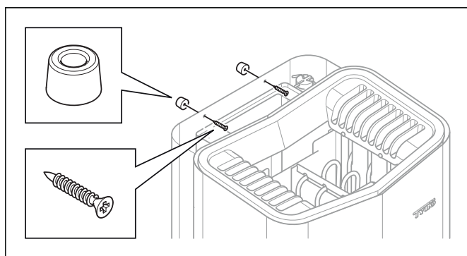
Fig 13: Fit spacers
