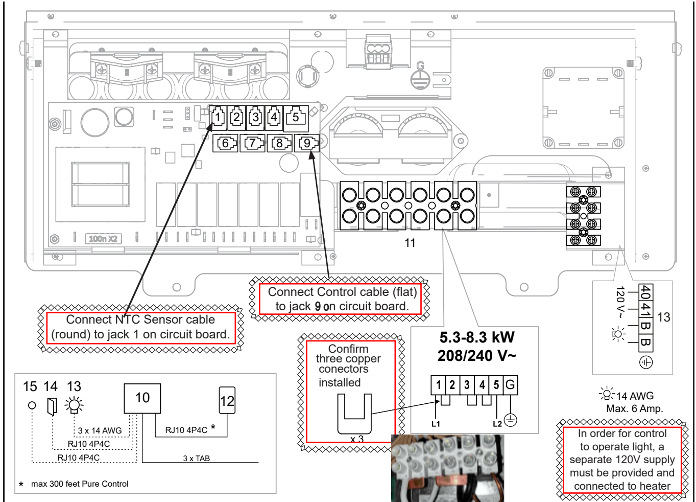
Figure 19: Wiring diagram
