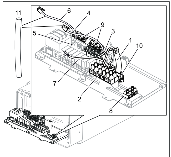
Figure 10: Circuit board
